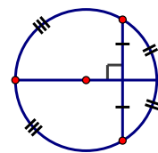
Diameters & Chords
