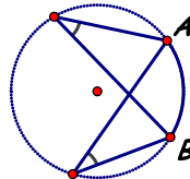
2 Inscribed Angles
