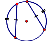
Chords & Arcs
