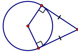
2 Tangents
