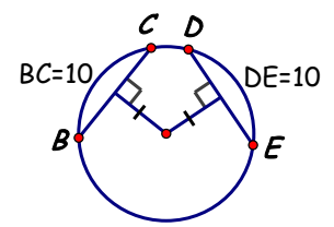
Congruent Chords
